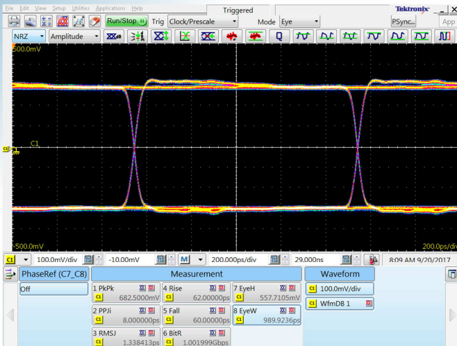
1 Gbps PRBS 2^{31}-1
