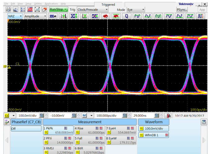
5 Gbps PRBS 2^{31}-1
