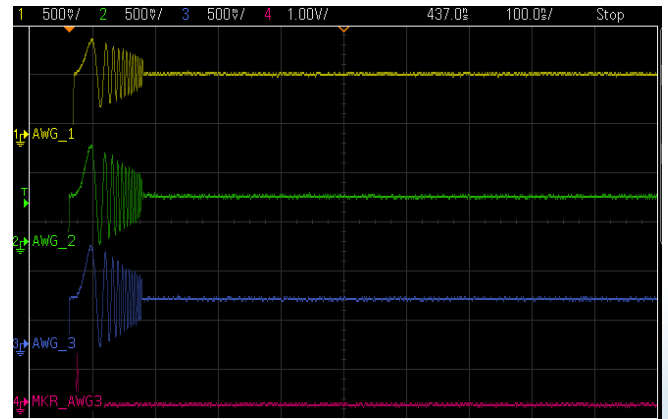
Burst mode of three synchronized SHF 19120 B
