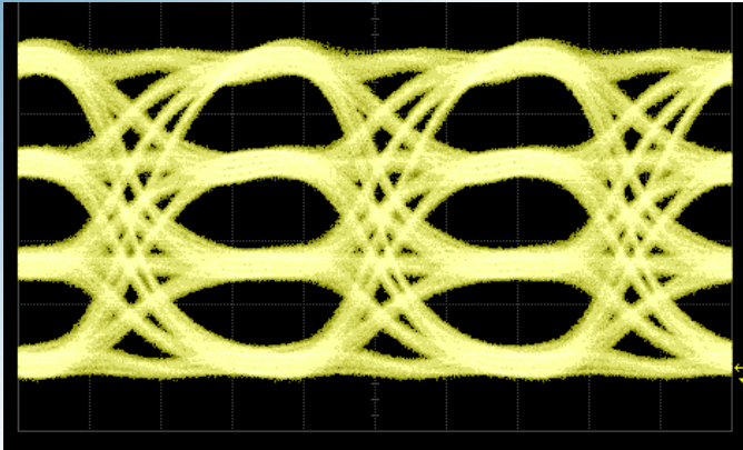
2.85 GSa/s PAM-4 signal, DC Output (200 mV/div ; 100 ps/div)
