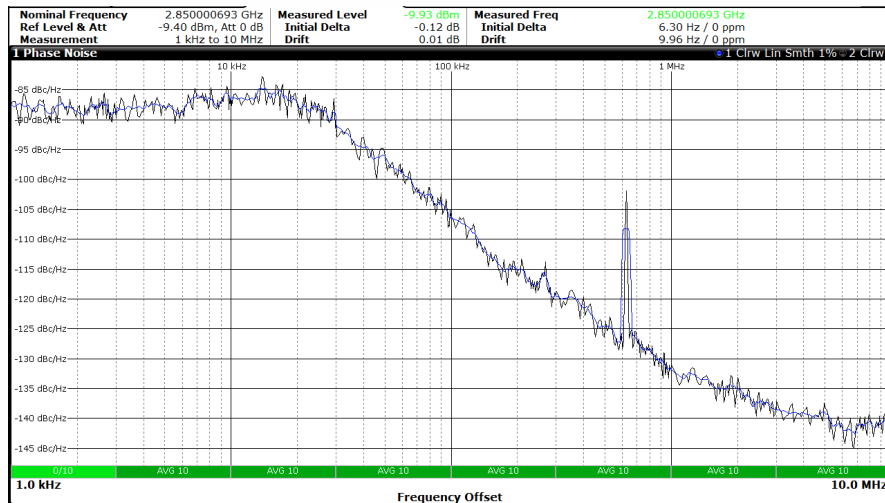
DAC Clock SMA Output, f_{DAC}=2.85 GHz
