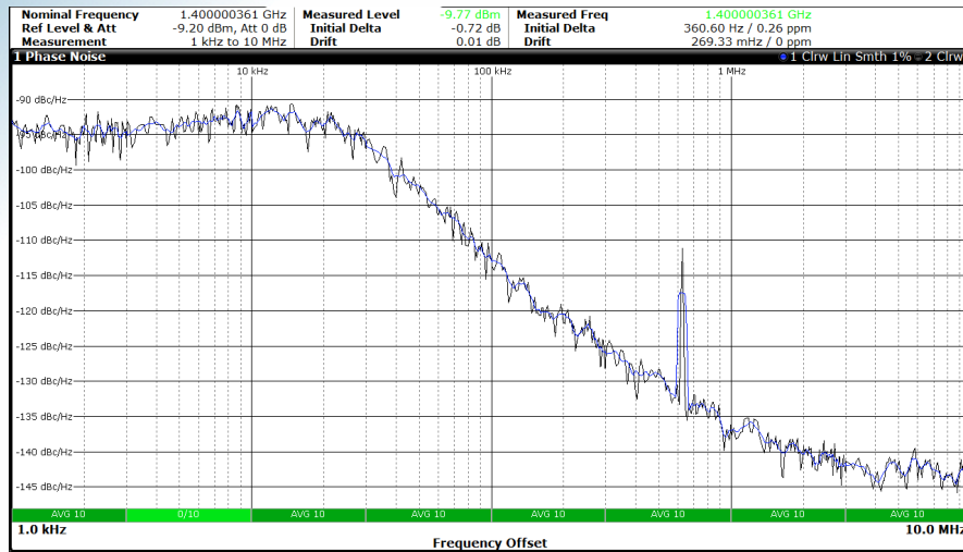
DAC Clock SMA Output, f_{DAC}=1.4 GHz
