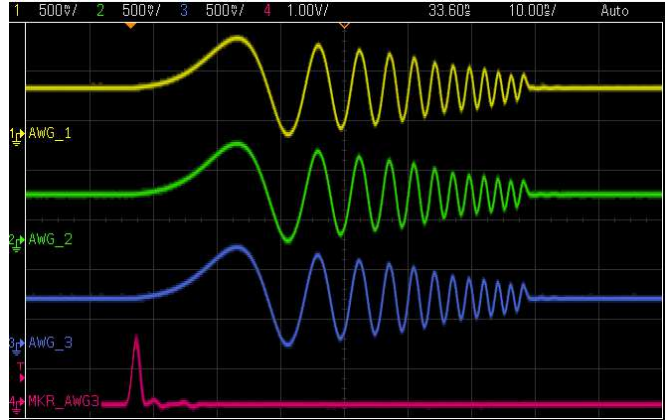
Frequency and phase synchronization of three SHF 19120 B
